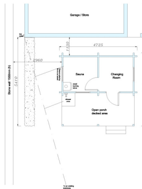
PROPOSED FLOOR PLAN
