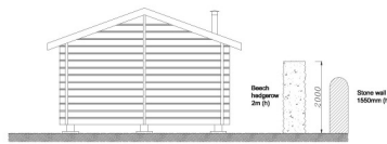
REAR ELEVATION (WEST)
