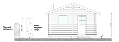
FRONT ELEVATION (EAST)
